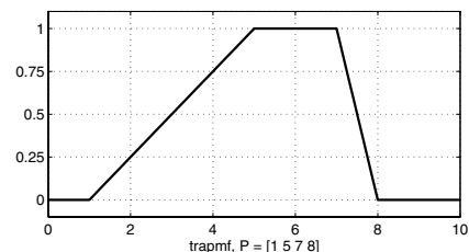
trapmf
